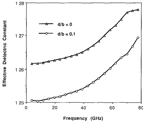
Fig. 4. Effects of sidewall mounting grooves on \epsilon_{\text{reff}}(\omega) for SSL's with w/b = 0.8 , d/b = 0 and 0.1 . ( a = 25 mil, b = 50 mil, h_2 = 5 mil).
