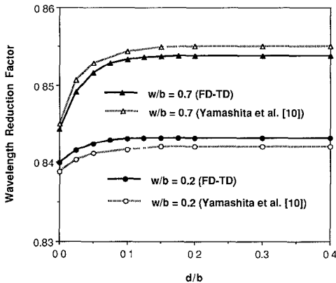
Fig. 5. Wavelength reduction factor \lambda/\lambda_0 versus groove depth calculated for SSL's with w/b = 0.2 and 0.7 at dc. ( a = 25 mil, b = 25 mil, h_2 = 5 mil).
